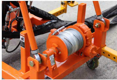
Wireline Hoist includes 500 ft. [152 m] of 1/8" [3.17 mm] of wire line cable.
