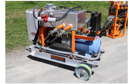
The hydraulic Power Pack consists of a 3-phase electric motor mounted to an aluminum skid.
