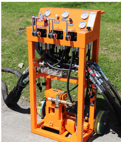
Modular Control Panel utilizes color coded quick disconnect hydraulic hoses for efficient breakdown and setup. A Quadraplex Piston Pump is conveniently mounted to the inside base of the Control Panel.
